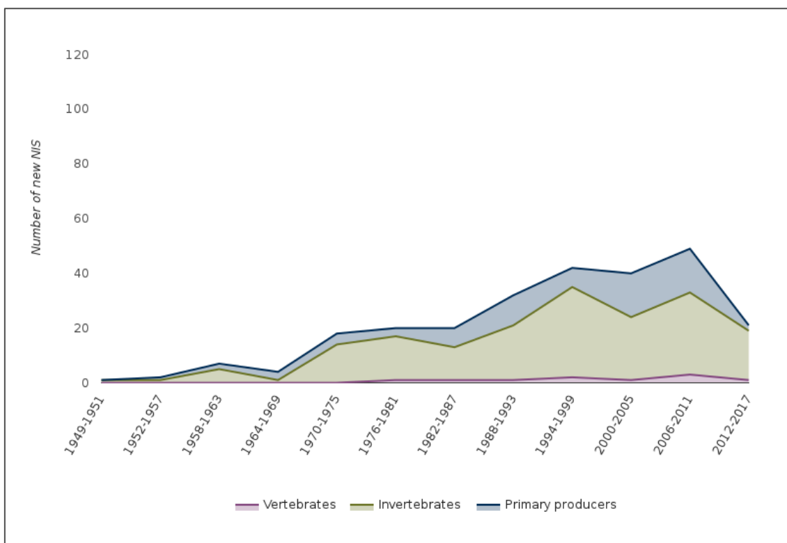
Figure 11: Temporal variability in numbers of new marine non-indigenous species per functional group, recorded in the North East Atlantic Sea.
