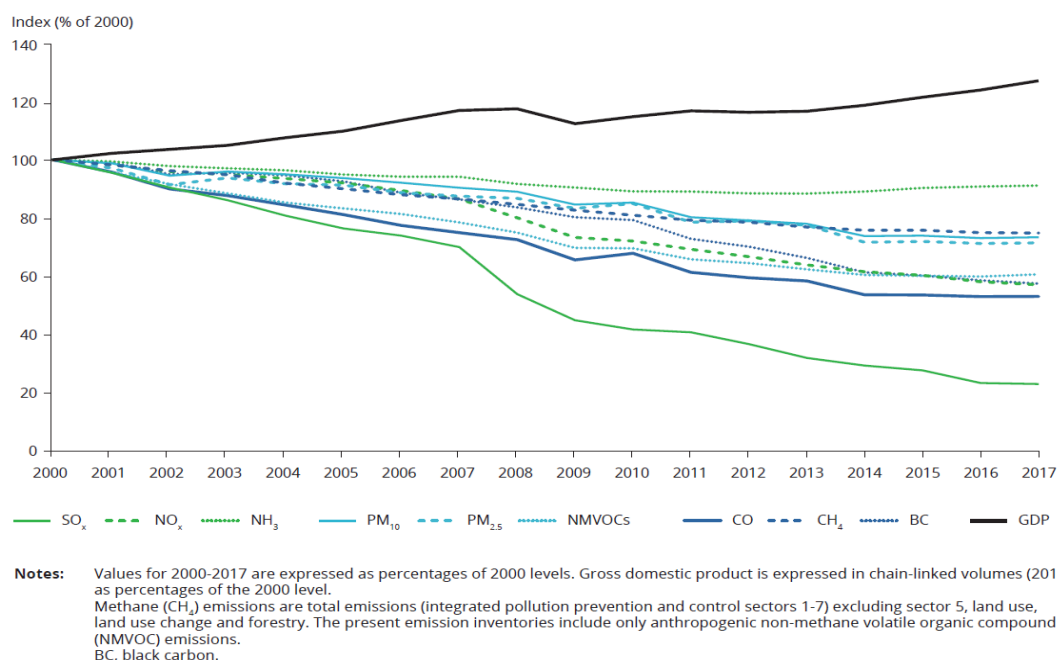
Figure 5: Trends in the main air pollutant emissions and in gross domestic product in the EU-27.
